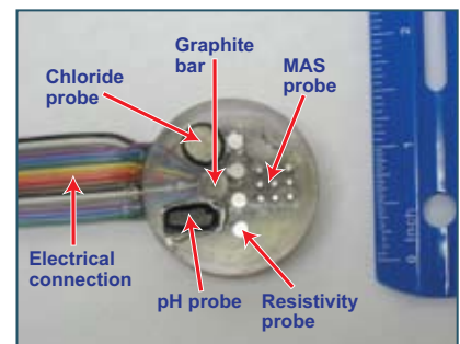
Concrete transducer prototype
