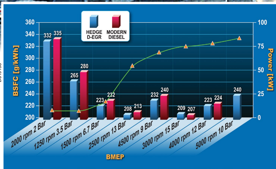
A fuel consumption comparison shows the relative performance parameters of a D-EGR engine and a modern diesel. (BSFC = brake specific fuel consumption, a measure of how much fuel is required to achieve a given power level.)
