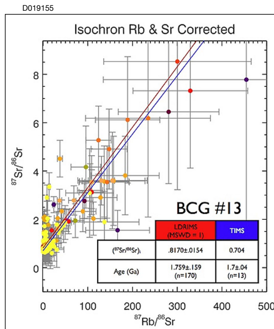
This isochron of a granite sample measured with LDRIMS-1 compares aging data derived by LDRIMS (red line) with traditional aging methods (blue line).
