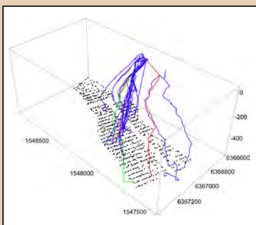
CNWRA scientists map pathways for radionuclide transport from potential geological repositories. Each pathway is color coded by calculated radionuclide discharge.
