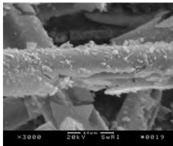
CNWRA scientists evaluated how the chemical degradation of submerged insulation materials may affect emergency cooling pumps in nuclear reactors after a loss-of-coolant accident.
