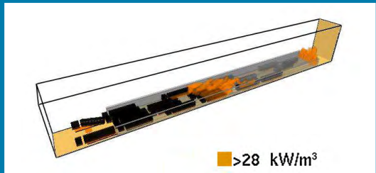
CNWRA simulated a major fire that occurred in a highway tunnel to evaluate the thermal conditions during the fire.
