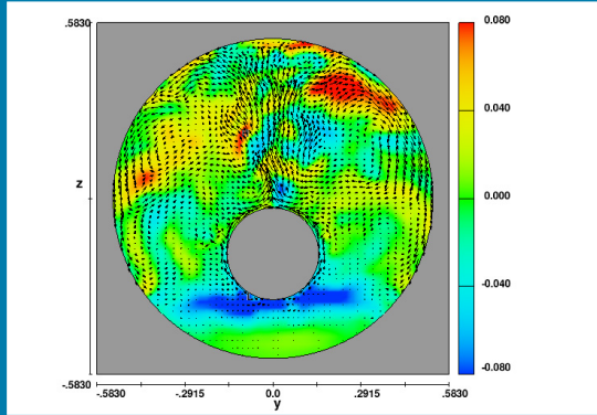
Using CFD simulations, CNWRA predicted the thermal and fluid flow processes that could take place in a high-level waste repository. These simulations establish confidence in full-scale drift modeling results under expected repository performance conditions.
