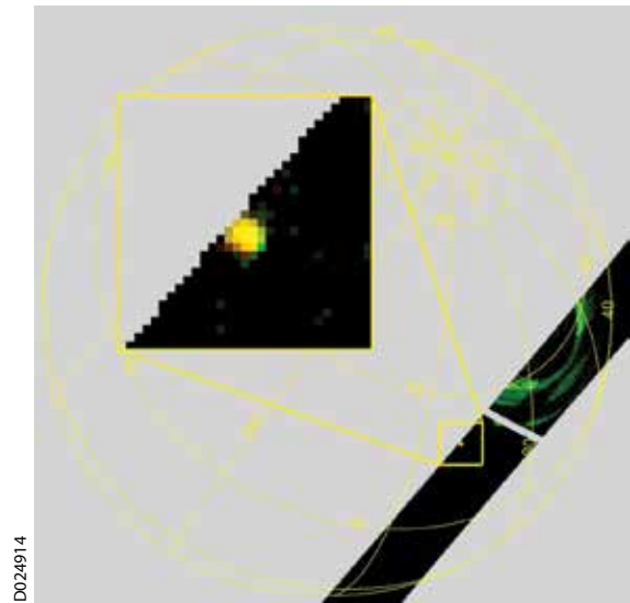
SwRI scientists studied the area imaged by Juno's UVS instrument on April 10, 2020, and determined that a large meteoroid had exploded in a bright fireball in Jupiter's upper atmosphere. The UVS swath includes a segment of Jupiter's northern auroral oval, appearing purely in green, representing hydrogen emissions. In contrast, the bright spot (see enlargement) appears mostly yellow, indicating significant emissions at longer wavelengths.
