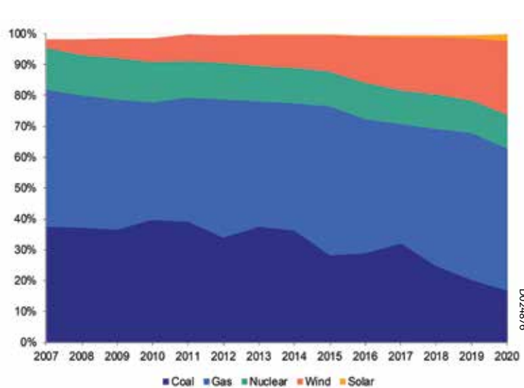
Many of SwRI's energy storage research projects are conducted in cooperation with Texas power generators. This graph shows the historic power generation mix for ERCOT, which manages the majority of Texas' power grid.
